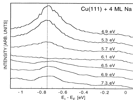
FIG. 1. Photoemission spectra recorded at different photon energies and along the surface normal from Cu(111) covered by 4 ML of Na.
