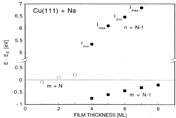
FIG. 4. Energy vs thickness in units of atomic Na layers, N , for quantum-well states with quantum number m=N (open squares) and m=N-1 (filled squares) in Na films on Cu(111), and final-state energies for intensity maxima (minima) observed for the emission from quantum-well states obtained when N is an odd (even) number.
