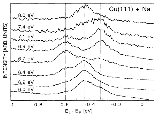
FIG. 2. Photoemission spectra recorded at different photon energies along the surface normal from Cu(111) covered with a Na film having an average thickness of 6 ML. The three peaks are due to quantum-well states characteristic of 5- (the peak at E - E_F = -0.58 eV), 6- ( -0.44 eV), and 7-ML-thick ( -0.32 eV) parts of the film.
