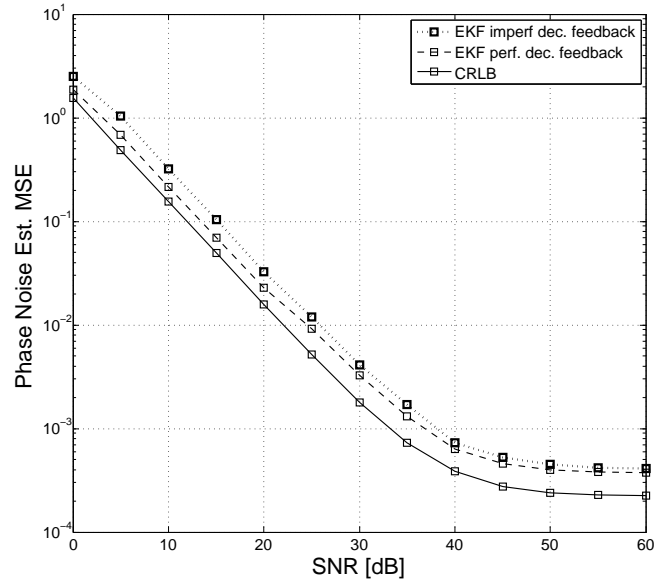
Fig. 7. Imperfect vs. perfect decision feedback MSE for DDE of phase noise for a 2 \times 2 MIMO system ( \sigma_{\Delta}^2 = 10^{-4} \text{ rad}^2 and L_p = 10 ).
