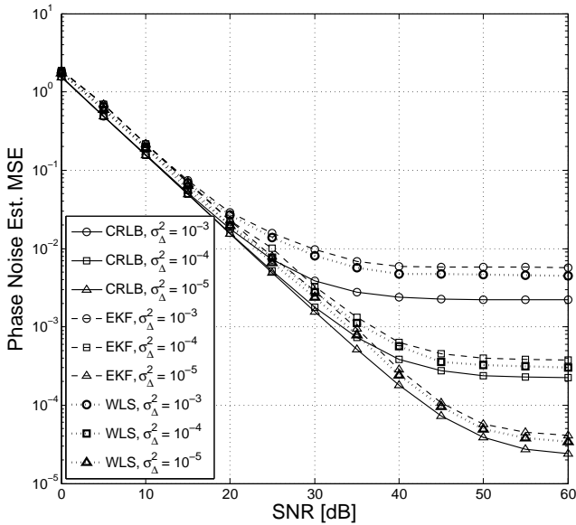
Fig. 6. Perfect decision feedback MSE for DDE of phase noise for a 2 \times 2 MIMO system for different phase noise variances.
