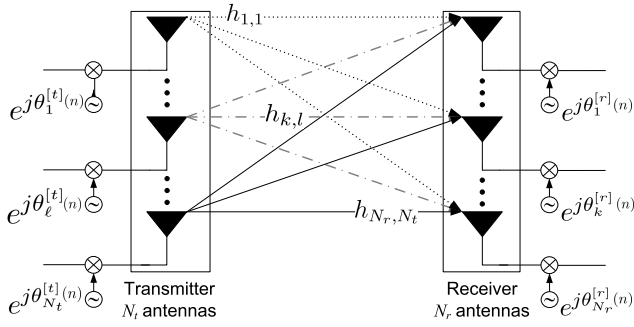
Fig. 1. System model for a point-to-point MIMO systems.
