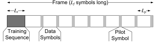
Fig. 2. Timing diagram for transmission of training, pilot, and data symbols within a frame.
