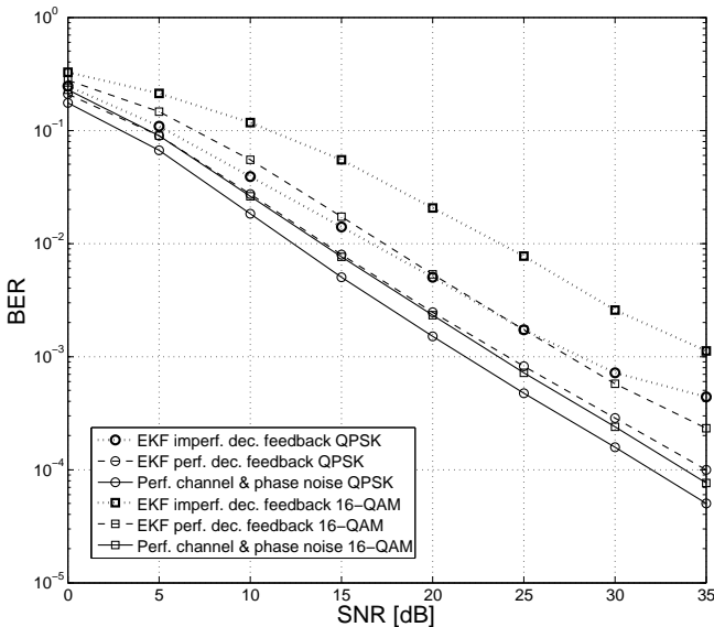
Fig. 10. BER of a 2 \times 2 MIMO system for QPSK and 16-QAM modulations ( L_p = 10 and \sigma_{\Delta}^2 = 10^{-4} rad 2 ).
