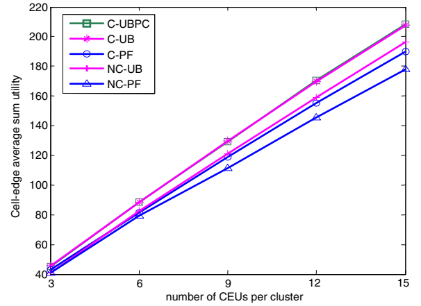
Figure 2. Average sum utility vs. number of CEUs per cluster
