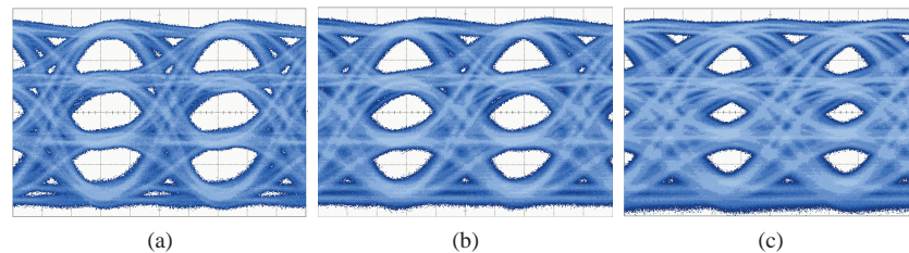
Fig. 2. Eye diagrams at 25 Gbps, after B2B (a) and after propagation over 200 m of MMF (b) and 300 m of MMF (c). The eye diagrams were taken at around 0 dBm received optical power.
