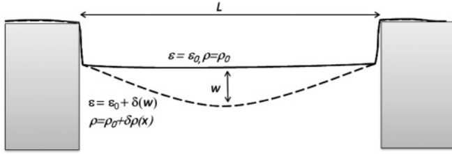
FIG. 2. Side view of suspended nanoribbon. In the text, a system where the ribbon is initially undeflected and has a finite induced 1D charge density \rho_0 and a built-in uniaxial strain \epsilon_0 . A deflection of magnitude w will induce an additional strain \delta(w) \sim w^2/L^2 as well as modify the charge distribution in the ribbon to \rho = \rho_0 + \delta\rho(x) .
