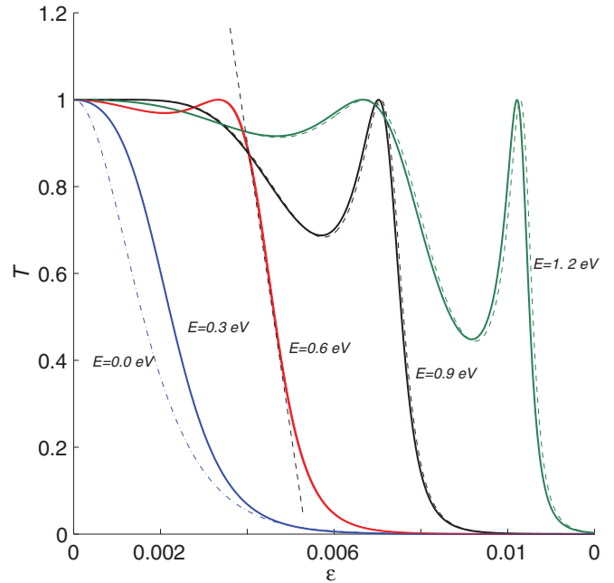
FIG. 4. (Color online) Transmission probability T through a metallic armchair ribbon ( W = 17 nm, L = 28 nm) [see Fig. 1(b)] as a function of strain \epsilon . T is shown as function of strain \epsilon for energies E = 0.0, 0.3, 0.6, 0.9, 1.2 eV. The slope of the straight dashed line determines the sensitivity of the working point around \epsilon = 0.5\% . The curved dashed lines show T corrected for displacement-dependent charge density (effective potential) for a ribbon with suspension height d_0 = 100 nm.
