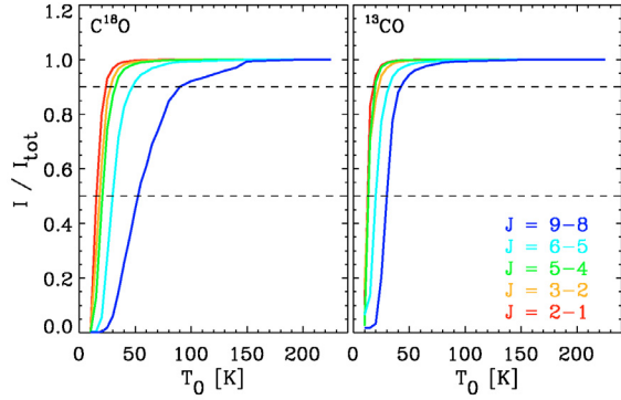
Fig. 3. Dependence of line intensities on temperature T_0 of C^{18}O (left) and ^{13}CO (right) for an “anti-jump” model of the CO abundance in the IRAS 2A envelope. The line intensities are measured relative to a model where the CO abundance is undepleted at all radii. Each curve therefore represents the fraction of the line intensity for the given transition, which has its origin in gas at temperatures below T_0 . The dashed lines indicate the levels corresponding to 50 and 90% respectively.
