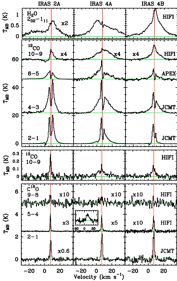
Fig. 1. Spectra at the central positions of IRAS 2A, 4A and 4B. Top to bottom: \text{H}_2\text{O} 2_{02}-1_{11} line from Kristensen et al. (2010) illustrating the medium and broad components, and spectra of ^{12}\text{CO} , ^{13}\text{CO} , and \text{C}^{18}\text{O} . The red lines correspond to the source velocities as obtained from the low- J \text{C}^{18}\text{O} lines. The insert in the \text{C}^{18}\text{O} 5–4 line for IRAS 4A illustrates the weak medium component with peak T_{\text{MB}} = 22 mK obtained after subtracting a Gaussian fit to the narrow line.
