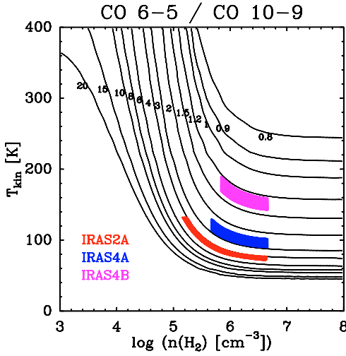
Fig. A.1. Model line ratios of CO 6–5/10–9 for a slab model with a range of temperatures and densities. The adopted CO column density is 10^{17} \text{ cm}^{-2} with a line width of 10 \text{ km s}^{-1} , comparable to the inferred values. For these parameters the lines involved are optically thin. The colored lines give the range of densities within the 20'' beam for the three sources based on the models of Jørgensen et al. (2002).
