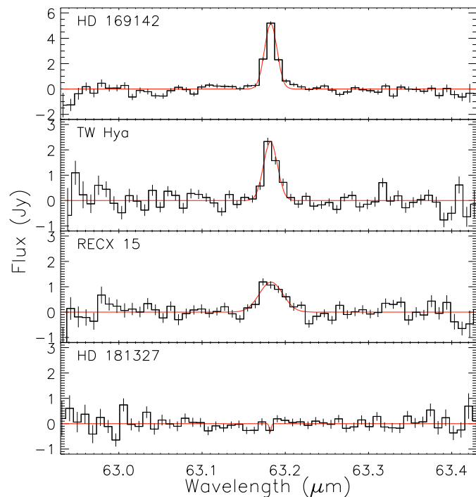
Fig. 1. Baseline subtracted, aperture and flux corrected [OI] 63 \mu\text{m} spectra. Error bars indicate 1\sigma statistical errors; gaussian line fits are shown in red.
