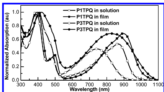
Figure 1. Absorption spectra of P1TPQ and P3TPQ in chloroform solution and in film.
