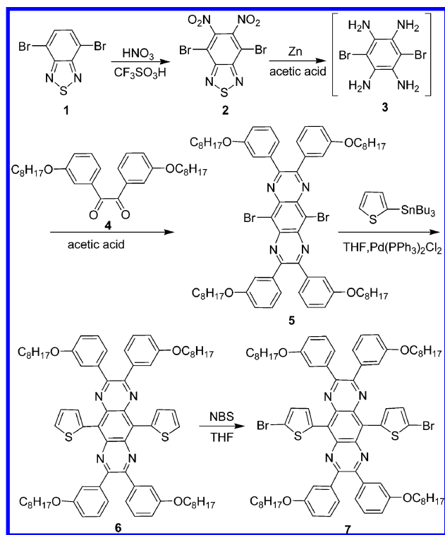
Scheme 1. Synthesis of the Two Monomers
