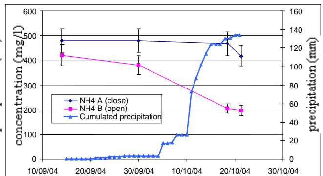
Figure 24 : Monitoring of the NH_4^+ concentration in the reservoirs A and B in Septembre-October 2004
