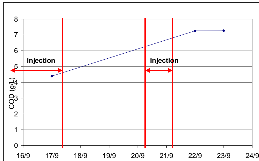
Figure 14: Monitoring of the COD at the exit of the bioreactor during the injection campaign
