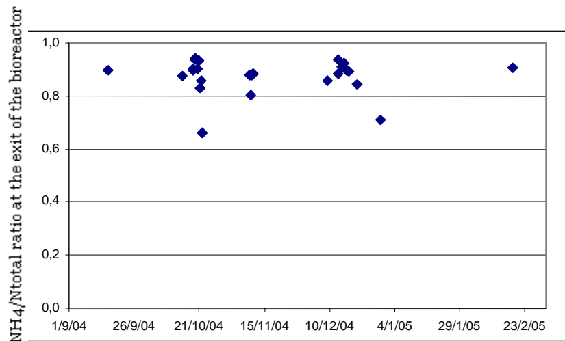
Figure 34: Evolution of the \text{NH}_4/\text{N}_{\text{total}} ratio
