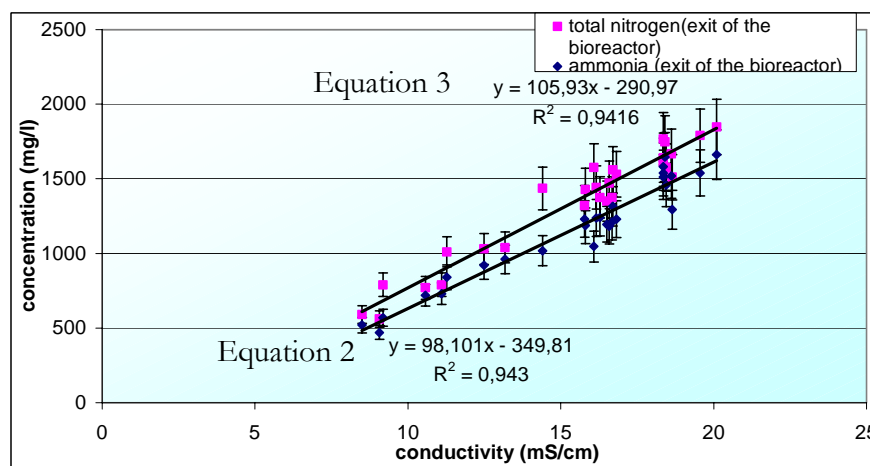
Figure 19 : Representation of total nitrogen and ammonia according to conductivity
