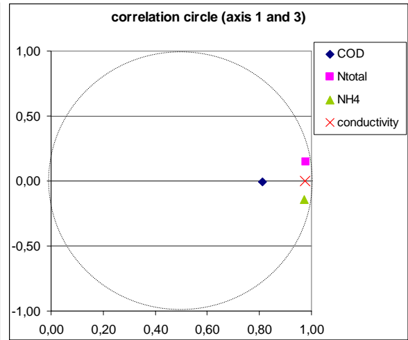
Figure 18 : Representation of the correlation circle on the principal axes 1 and 3 (*)
