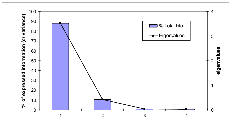
Graph 1 : Eigenvalues and their respective weights
