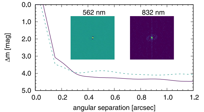
Figure 4. Contrast curves calculated from our WIYN/NESSI speckle images (inset). The green curve corresponds to the 562 \text{ nm} image, and the purple curve to the 832 \text{ nm} image. Each of the reconstructed images is \approx 1.2 \text{ arcsec} \times 1.2 \text{ arcsec} in size.
