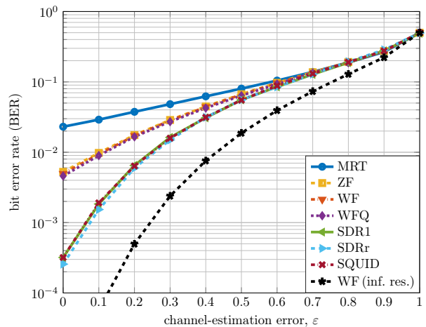
Fig. 5. Uncoded BER with QPSK signaling for 1-bit DACs as a function of the channel-estimation error, \varepsilon .
