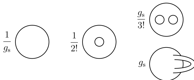
Figure 2.3: Leading-order open world-sheet components with g_s weights and symmetry factors for exchanging identical boundaries: a disk, an annulus, a disk with two holes, and a disk with a handle. All boundaries are attached to a single point in space-time.
