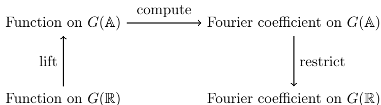
Figure 1.1: Illustration of the computation of Fourier coefficients on G(\mathbb{R}) by first lifting to the adèles.
