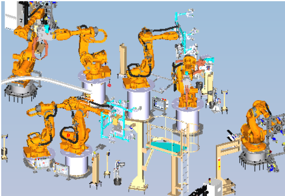
Figure 6.1: The seven robots in the provided robot cell.
