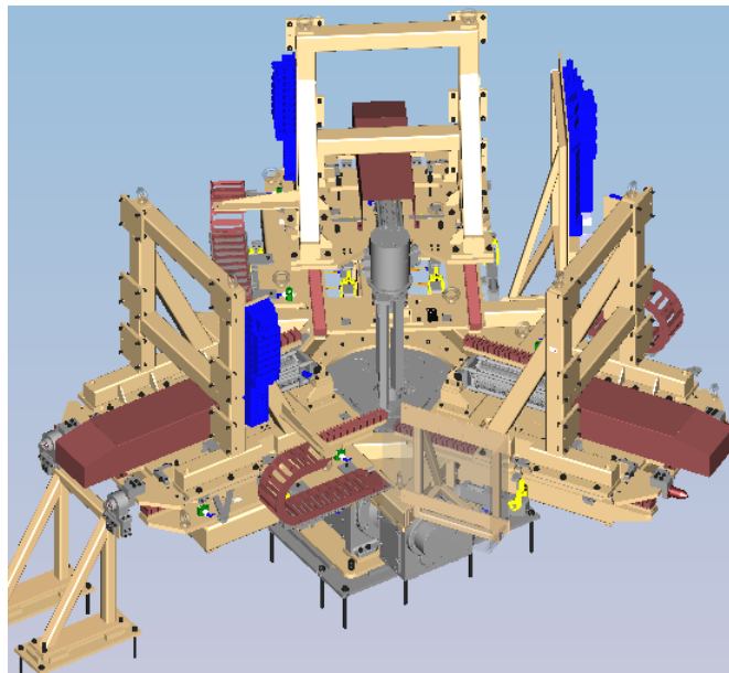
Figure 6.3: One of the two turntables from the provided robot cell.
