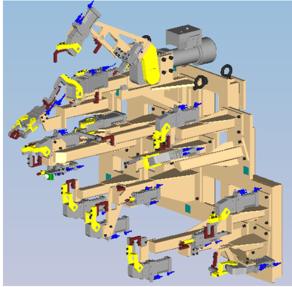
Figure 6.2: Sample fixture from the provided robot cell.
