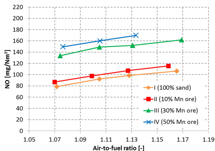
Figure 7. Measured concentrations of NO ( \text{mg}/\text{Nm}^3 , at 6% \text{O}_2 ) at position kh2 in the convection path as a function of the air-to-fuel ratio for experiments with partial substitution of sand with manganese ore.
