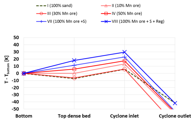
Figure 4. Temperature profile over the boiler when operated on higher air-to-fuel-ratio ( \approx 1.17 ). T_{\text{bottom}} was in the range 855–875 °C and have been used as reference. For 50% Mn ore, data were for air-to-fuel ratio 1.13 since data for 1.17 are lacking.
