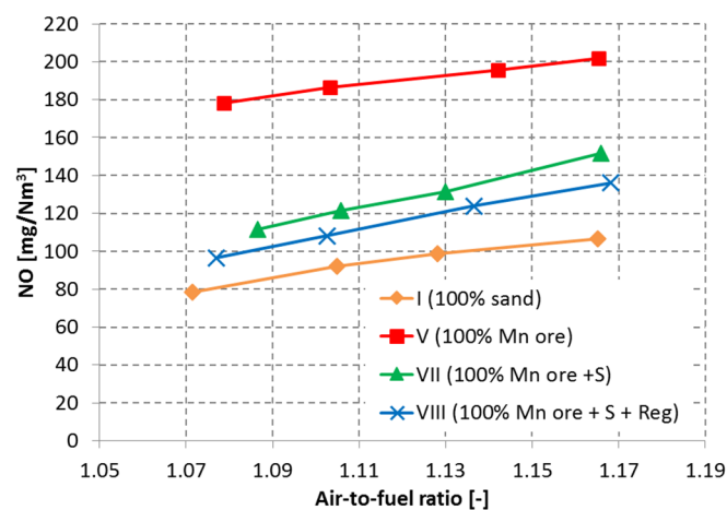
Figure 8. Measured concentrations of NO ( \text{mg}/\text{Nm}^3 , at 6% \text{O}_2 ) at position kh2 in the convection path as a function of the air-to-fuel ratio for experiments with 100% manganese ore.
