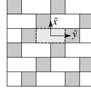
Figure 5: A pattern matrix with a highlighted yarn segment in the center. The corresponding yarn local coordinate system is also illustrated. The y-axis is defined such that it always runs along the yarn, while the x-axis runs across it.
