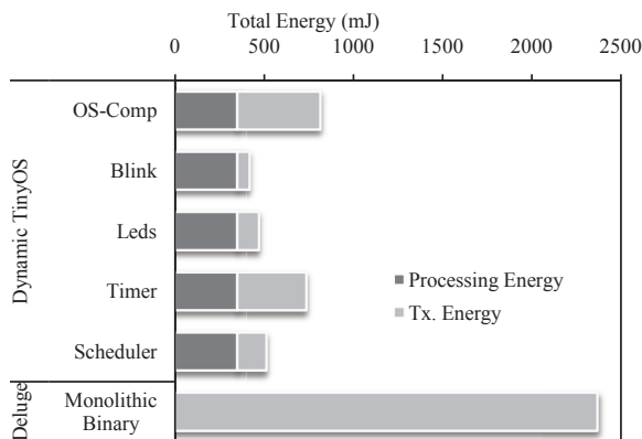
Figure 10 Energy overhead comparison of DyTOS with Deluge. DyTOS results in significantly less overhead than Deluge for all the update scenarios. Deluge has a constant overhead for all update scenarios
