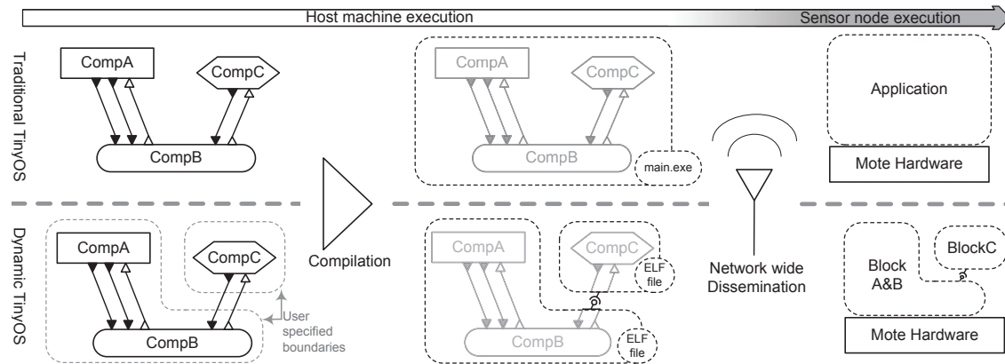
Figure 1 Overview of code updates in DyTOS in comparison with the traditional TinyOS: In the first step a user chooses boundaries among the building blocks of an application and the OS. In the second step, ELF files are generated according to the specified boundaries. These ELF file are disseminated in the network and linked on the mote to form the application
