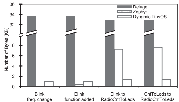
Figure 7 Performance in common software update scenarios. Zephyr results in smaller updates for very small changes in application. In contrast, DyTOS has a stable update-size because it operates at the component level. It outperforms Zephyr in the case of bigger changes in applications such as the addition of a new component
