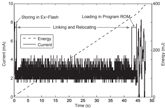
Figure 9 Current draw and energy utilisation during processing and loading of the BlinkTask application on the TelosB platform. The peaks, generated by turning on all onboard LEDs simultaneously, mark the boundaries between the different operations
