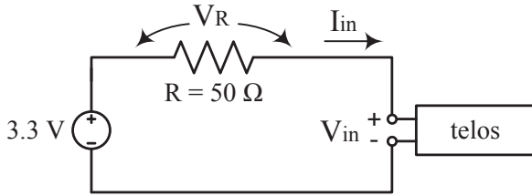
Figure 5 Current measurement setup
