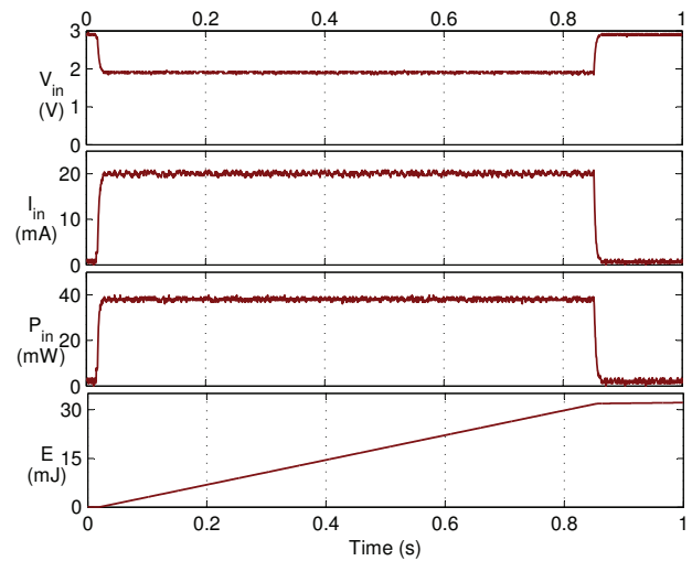
Figure 6 Input current, instantaneous power and energy consumption during the transmission of 3000 bytes with the telos platform (see online version for colours)
