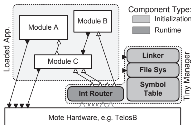
Figure 2 Architectural elements of Tiny Manager . Only the interrupt router is active during the normal execution of a loaded application. Linker, file system and symbol table handle storage and integration of newly received code
