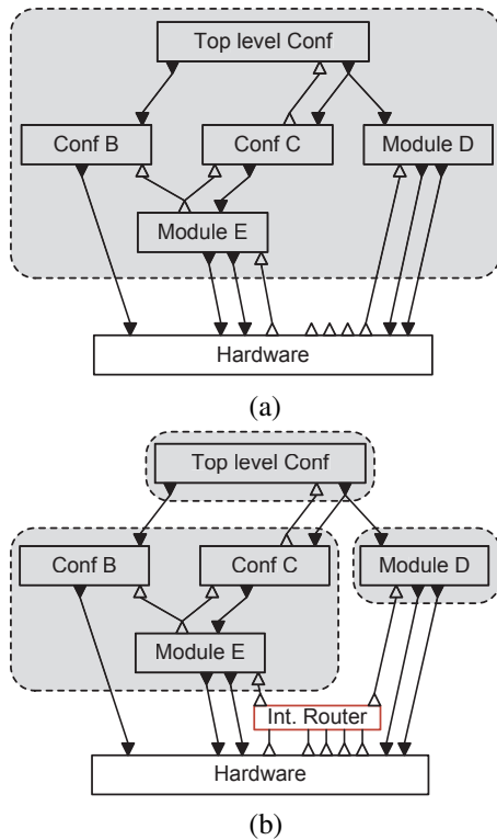
Figure 3 Internal structure of a TinyOS application: (a) TinyOS and (b) DyTOS (see online version for colours)
