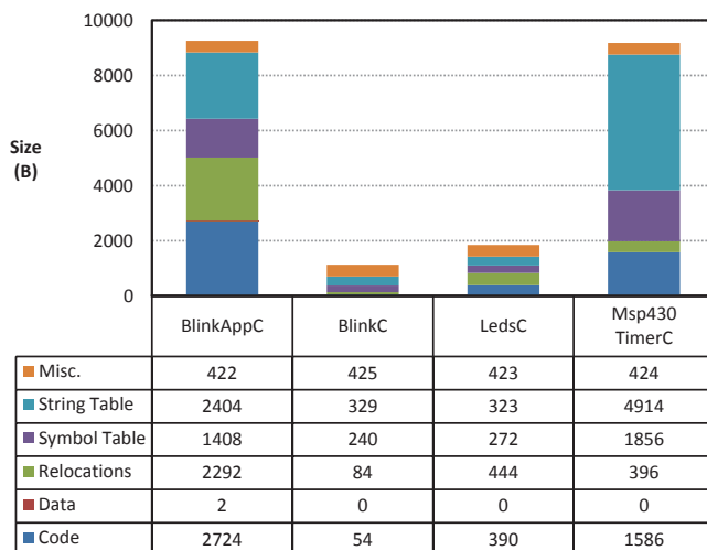
Figure 4 Breakdown of contribution from different sections of ELF file toward its total size. The string table included in these files is the main contributor toward their size and hence is primary candidate for optimisation. These ELF objects belong to the trademark Blink application a from TinyOS repository (see online version for colours)
