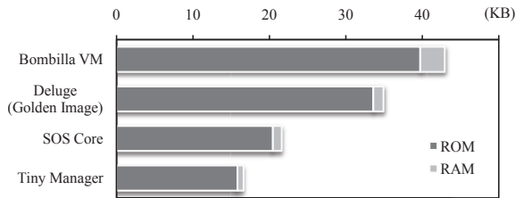
Figure 8 Memory-footprint comparison for DyTOS . Tiny Manager only utilises 7.7% of the RAM and 32% of the internal flash ROM on TelosB platform, which is significantly less than all other comparable solutions
