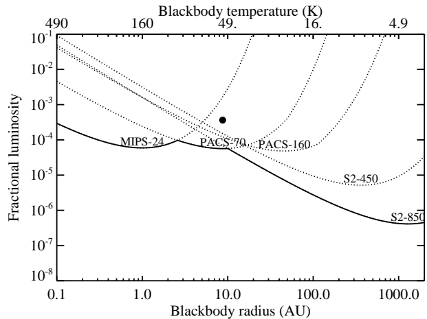
Figure 1. Relative sensitivities of Spitzer MIPS ( 24 \mu\text{m} ), Herschel PACS and SCUBA-2 to dust emission at the level of AU Mic’s disk, shown as a black dot. Any disk above each instrument’s sensitivity curve will be detectable to that instrument. The best fit temperature and fractional luminosity of AU Mic render undetectable to MIPS at 24 \mu\text{m} (as reported by Chen et al. 2005), but detectable to PACS at 70 and 160 \mu\text{m} as well as SCUBA-2 at 450 and 850 \mu\text{m} .
