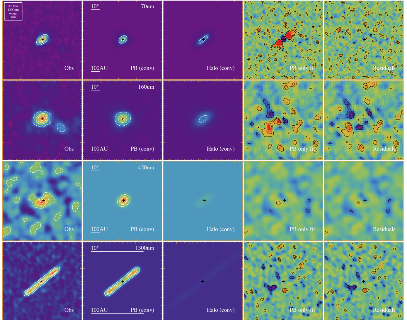
Figure 6. Resolved images of the AU Mic disk at (top to bottom) 70\ \mu\text{m} , 160\ \mu\text{m} , 450\ \mu\text{m} and 1300\ \mu\text{m} (left column, as in Figure 2) compared to the planetesimal belt (second column) and halo (third column) components. The fourth column shows residuals (and \pm 2 - and 3 - \sigma contours) when only the planetary belt model (multiplied by 1.8, 1.4, 1 and 1 for 70, 160, 450 and 1300\ \mu\text{m} , respectively) is removed from the data and the fifth column shows the residual when the full (parent belt + halo) model is subtracted from the data, and includes additional background components, which are most visible in the 160\ \mu\text{m} image. The color scale for the first three panels along each row is the same to show the relative contribution of each component. The color scale on each row is different, scaled to near the peak flux in the observed image at that wavelength. The color scale of the residual images are scaled to the same \pm\sigma level. While the residuals at 450\ \mu\text{m} are suggestively symmetric, they are not aligned with the known disk orientation and are barely at the 2 - \sigma level. In addition, a point source at the stellar position was included in the model at 1.3\ \text{mm} , consistent with the unresolved excess reported by MacGregor et al. (2013). The residual to the south of the star at 1.3\ \text{mm} is assumed to be an unrelated background source.
