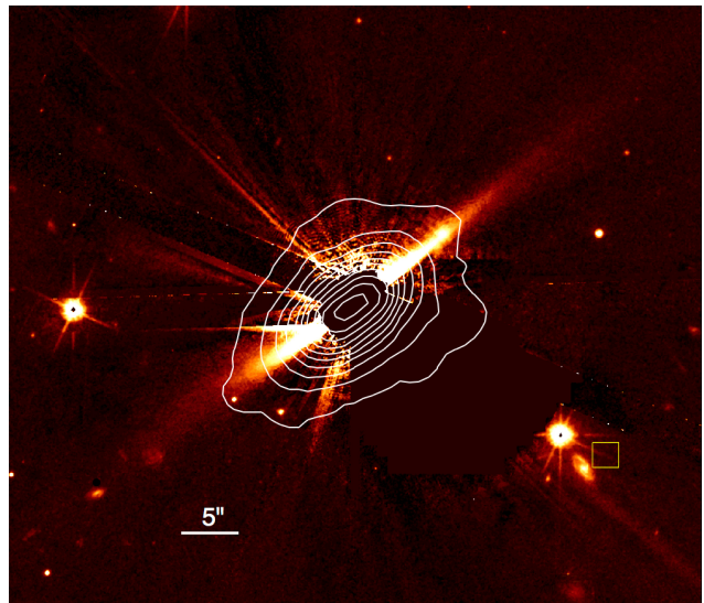
Figure 4. Optical image of AU Mic from HST showing the orientation and extent of the scattered light disk. North is up and east is to the left. The 70\ \mu\text{m} emission from Herschel is overlaid. The disk is clearly resolved at 70\ \mu\text{m} , and the disk orientations are consistent, to the limits of the Herschel resolution. The yellow box shows the position of the 70\ \mu\text{m} source detected with Herschel at the epoch of the HST observations. The position is close to, but not coincident with, the optically visible galaxy approximately 2'' to the southeast.
