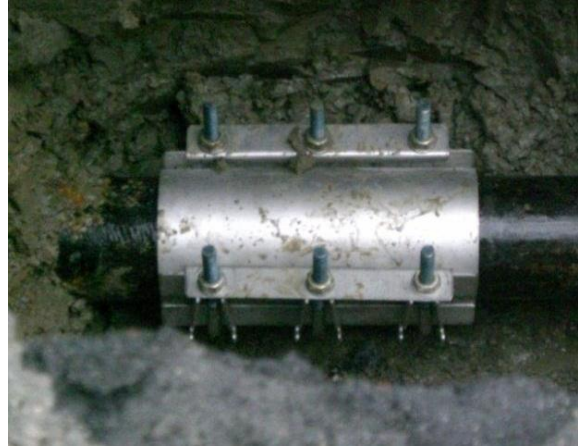
Figure 5 Grey cast iron pipe failure Type A (left), easily repaired with a repair clamp (right). Photo Annika Malm.
