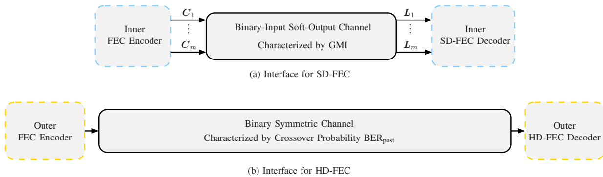
Fig. 2. Interface for (a) the inner SD-FEC and (b) the outer HD-FEC in Fig. 1 (for one polarization). The BISO channel characterized by the GMI and the BSC by its crossover probability given by the BER after SD-FEC decoding \text{BER}_{\text{post}} .
