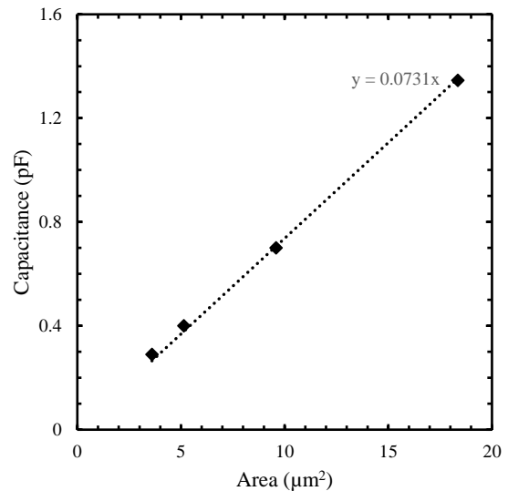
Fig. 2. The measured capacitance values for SIS junction with four different areas using [10]. The linear trendline shows the specific capacitance of 73.1 \text{ fF}/\mu\text{m}^2 .
