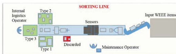
Fig. 2. Hypothesis of layout and components of the automated sorting line.
