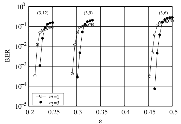
Fig. 1. BER performance of nonbinary SC-LDPC codes for m = 1 and 3.
