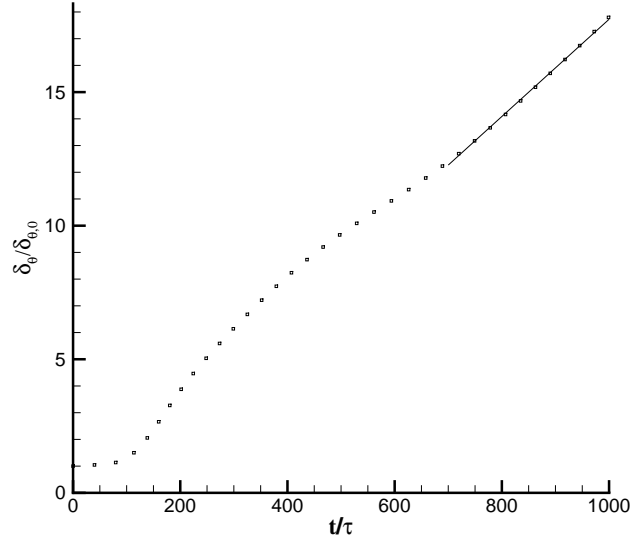
Figure 2: Time evolution of momentum thickness for M_c = 0.3 .
