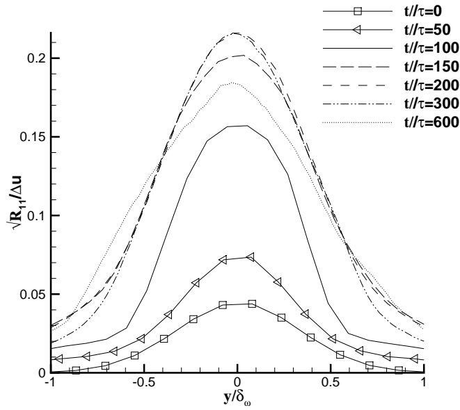
Figure 3: Time evolution of \sqrt{R_{11}} .
