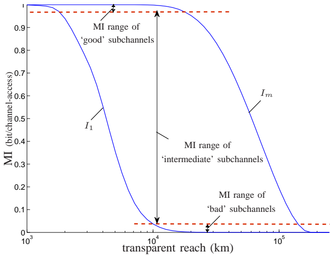
Fig. 2. A schematic example of bitwise conditional MIs together with the range of MIs for the ‘good’, ‘intermediate’, and ‘bad’ groups.
