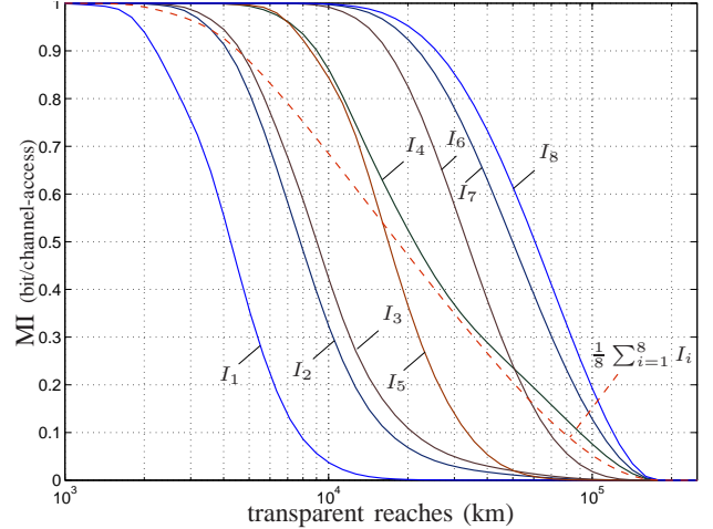
Fig. 4. The bitwise conditional MIs for a 4D mapper with PM 16-QAM. The fiber-optic link is implemented with the parameters given in Table I.
