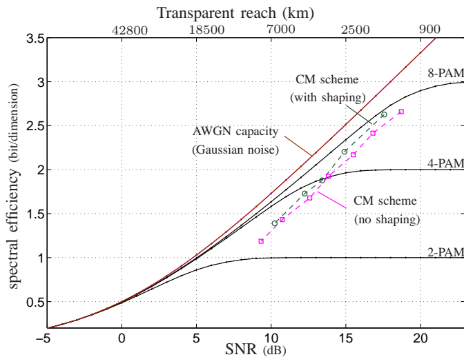
Fig. 8. The spectral efficiency per dimension versus the transparent reach and the SNR for a non-DM link with EDC. The CM scheme curves are based on the results given in Tables V and IV and the spectral efficiency for the Gaussian noise model is computed by (1/2)\log_2(1 + \text{SNR}) , where \text{SNR} = |\zeta|^2 P / \sigma_{Z_x}^2 .
