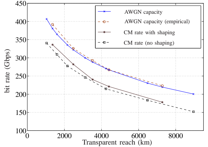
Fig. 7. Bit rates per two polarizations achieved by the CM scheme versus the transparent reach of a non-DM link with EDC, with and without probabilistic shaping.
