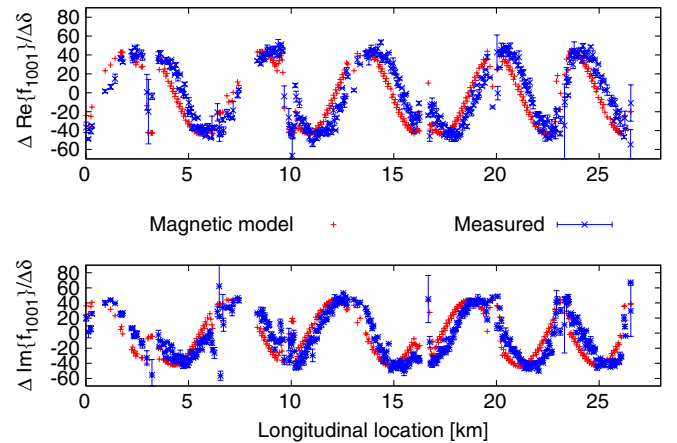
FIG. 3. Comparison between the measured chromatic coupling (blue) and the expected chromatic coupling from our magnetic model (red). This is for beam 2 at 4 TeV, with a \beta^* of 60 cm.
