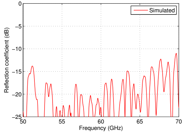
Fig. 10. Simulated reflection coefficient of the SWE antenna.
