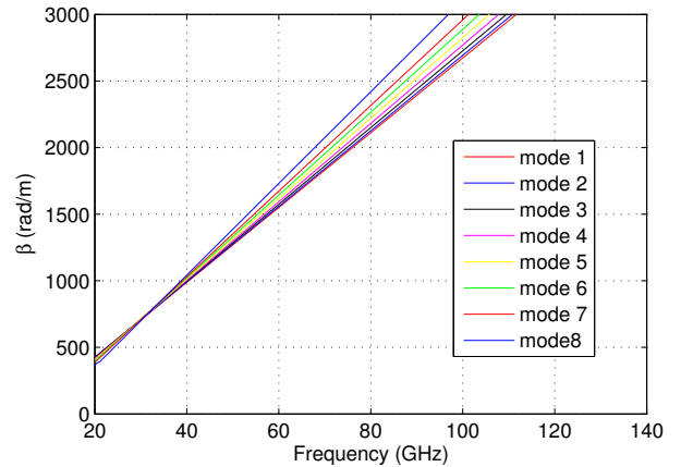
Fig. 4. Dispersion diagram of the sheet waveguide ( 140 \times 0.3\text{mm}^2 ).
