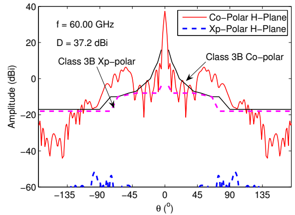
Fig. 12. Simulated radiation patterns in E- and H-plane at 60 GHz.
