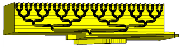
Fig. 8. Feeding network.
