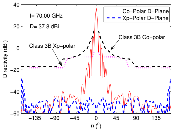
Fig. 11. Simulated radiation patterns in 45° plane.
