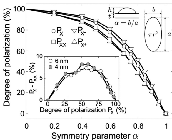
FIG. 3. Computed degree of linear polarization for the exciton P_X (circles), biexciton P_{XX} (squares), positive trion P_{X+} (up-pointing triangles), and negative trion P_{X-} (down-pointing triangles) as a function of the symmetry parameter \alpha , keeping r = 6 nm. The top inset shows a schematic illustration of the QD model, and the lower inset shows the computed difference in degree of linear polarization between the exciton and the biexciton for two QD sizes ( r = 6 nm and r = 4 nm), plotted versus the polarization degree of the exciton emission. Solid lines serve as guide to the eye.
