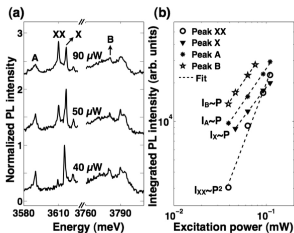
FIG. 1. (a) \mu PL spectra of GaN QDs measured with different excitation power, as indicated in the figure. (b) The integrated peak intensity of the emission lines XX, X, A, and B versus the excitation power.
