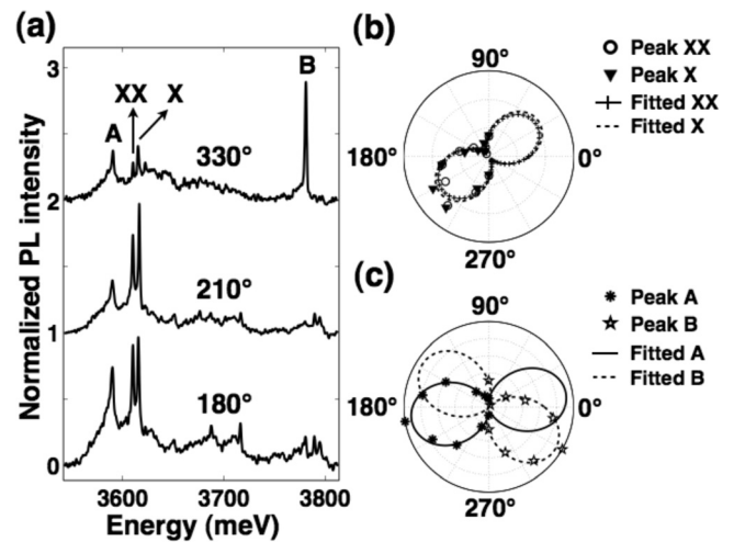
FIG. 2. (a) Polarization resolved \mu PL spectra of GaN QDs recorded for different angles 180^\circ , 210^\circ , and 330^\circ of the linear polarization analyzer. (b), (c) Polar plots of the integrated peak intensities of the emission lines XX, X, A, and B as a function of the polarization analyzer angle along with curve fittings.
