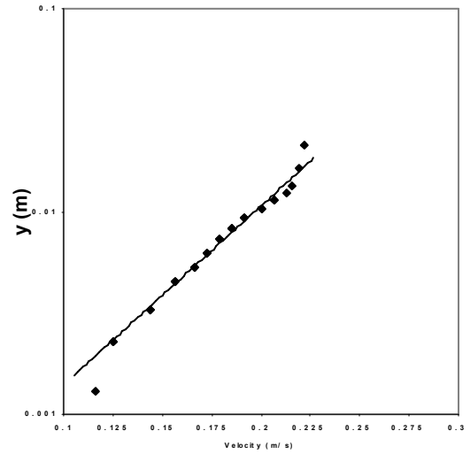
Velocity profile 2
