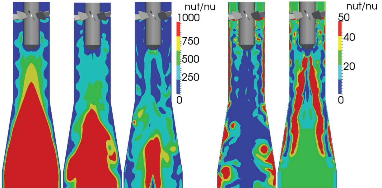
Figure 3.4.5: Slice in the x or y plane of the Swirl Generator colored by the ratio of the turbulent kinematic viscosity to the molecular kinematic viscosity. From left to right: k-\epsilon , k-\omega SST, k-\omega SST SAS, Spalart-Allmaras DDES and Spalart-Allmaras IDDES.
