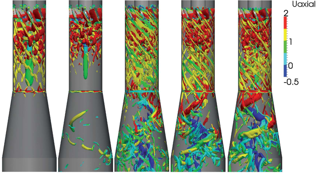
Figure 3.3.6: Isosurface of the second invariant of the velocity gradient tensor (colored by axial velocity in [\frac{m}{s}] ). The axial velocity is positive in flow direction, i.e. from top to bottom. From left to right: k-\epsilon , k-\omega SST, k-\omega SST SAS, Spalart-Allmaras DDES and Spalart-Allmaras IDDES.
