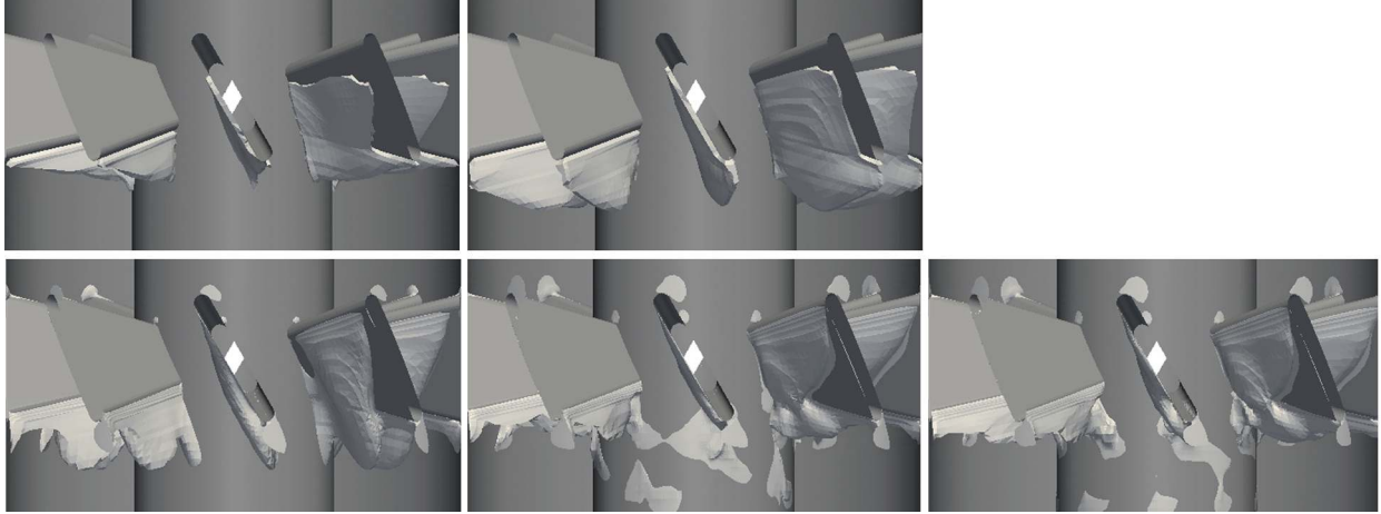
Figure 3.4.7: Separation around the blades visualized by an isosurface of axial velocity equal to -0.001 \frac{m}{s} . Upper row: RANS models from left to right: k-\epsilon , k-\omega SST; lower row: hybrid models from left to right: k-\omega SST SAS, Spalart-Allmaras DDES, Spalart-Allmaras IDDES.
