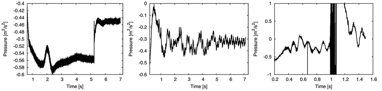
Figure 3.3.1: Development of the pressure signal at position P1. From left to right: k-\epsilon , k-\omega SST and k-\omega SST SAS.
