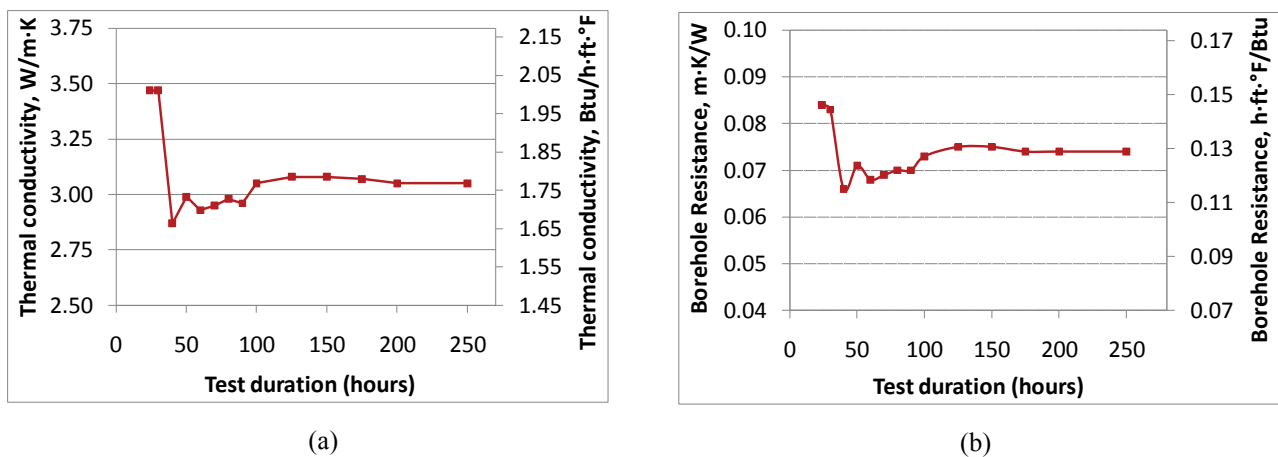
Figure 2 Ground thermal conductivity and borehole thermal resistance estimations for different test lengths of borehole 3.
