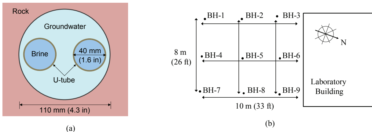
Figure 1 Geometry and layout of the laboratory boreholes.
