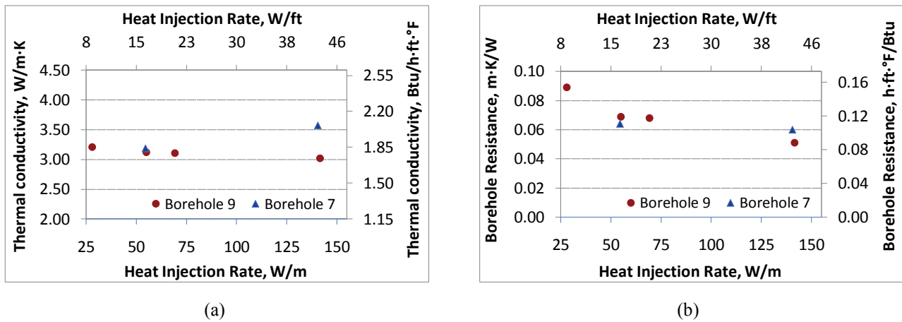
Figure 3 a) Ground thermal conductivity and b) borehole thermal resistance estimations for different heat injection rates for boreholes 7 and 9.
