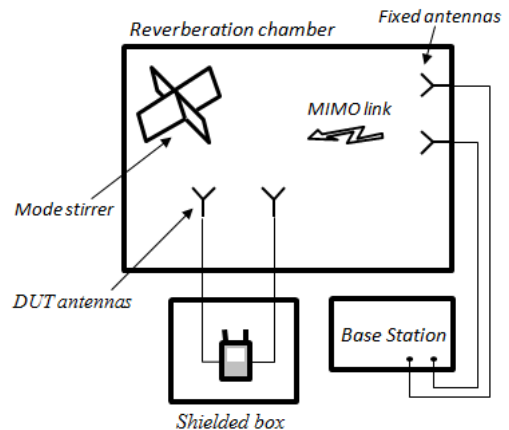
Fig. 3 Using the reverberation chamber for LTE throughput measurement with external antennas connected to the DUT. Note that the DUT is placed in a separate shielded box.
