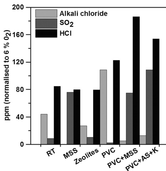
Fig. 4 – Flue gas concentration before the convection pass.
