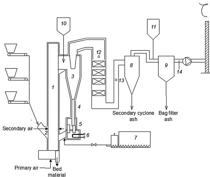
Fig. 1 – Schematic figure of the 12 MW th circulation fluidised bed boiler.
