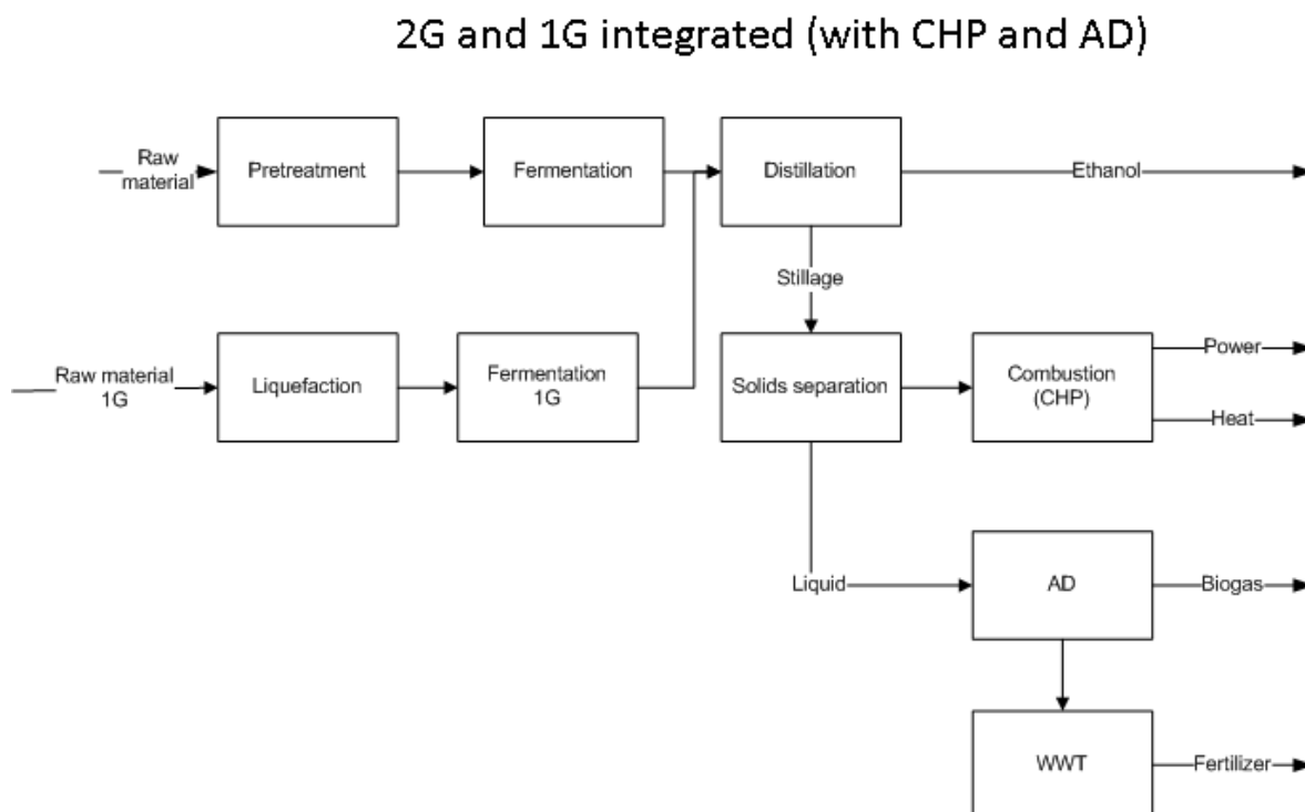
Figure 4.2. Integration between the production of the second and first generation ethanol.
