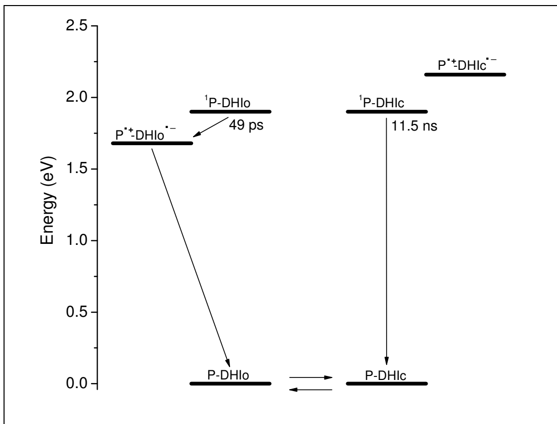
Figure 2. Transient states and relevant interconversion pathways for dyad 1 with the photochromic moiety in the open, 1o , form (left) and the closed, 1c , form (right).
