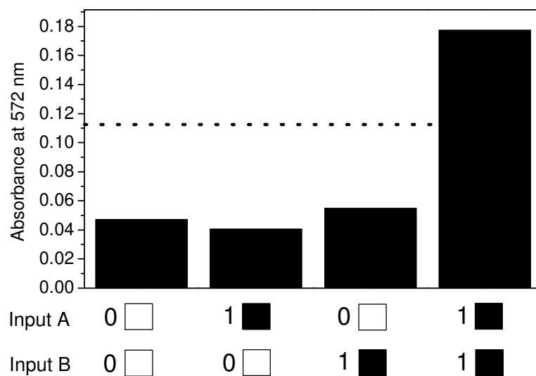
Figure 4. Performance of dyad 1 in the AND gate mode. The bars show the absorbance measured at 572 nm after each input combination (see text for details). The dotted line represents an arbitrarily set threshold level to distinguish output on from output off . Before each input combination, the sample was reset to the initial 1a state using red light.
