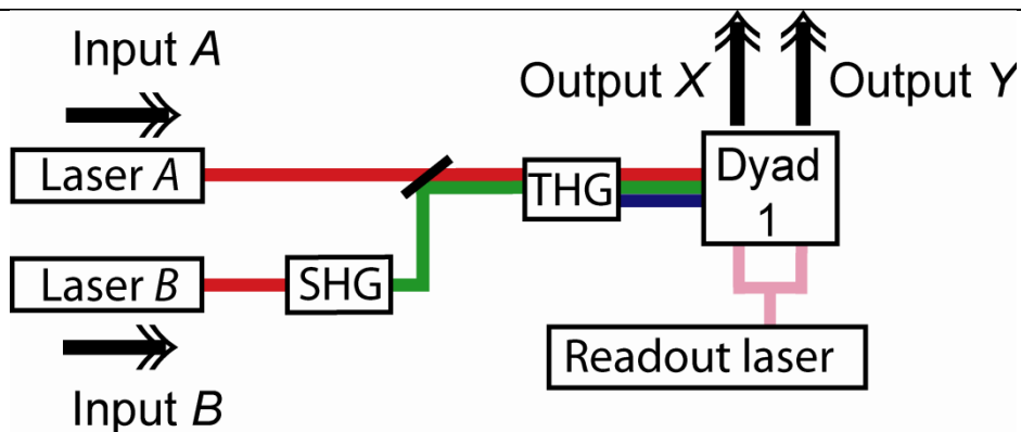
Figure 3. Schematic sketch showing how to implement AND and NAND gate functions using dyad 1 and a third-harmonic-generating crystal (THG). Lasers A and B are pulsed Nd:YAG lasers at 1064 nm. Switching laser B on will produce 532 nm light (via a second-harmonic generating crystal, SHG). Switching both lasers on simultaneously will produce 355 nm UV light (via the THG). The absorbance at 572 nm (AND gate, output X) and the emission at 722 nm (NAND gate, output Y) of dyad 1 are monitored by a readout laser and suitable diodes for detection.
