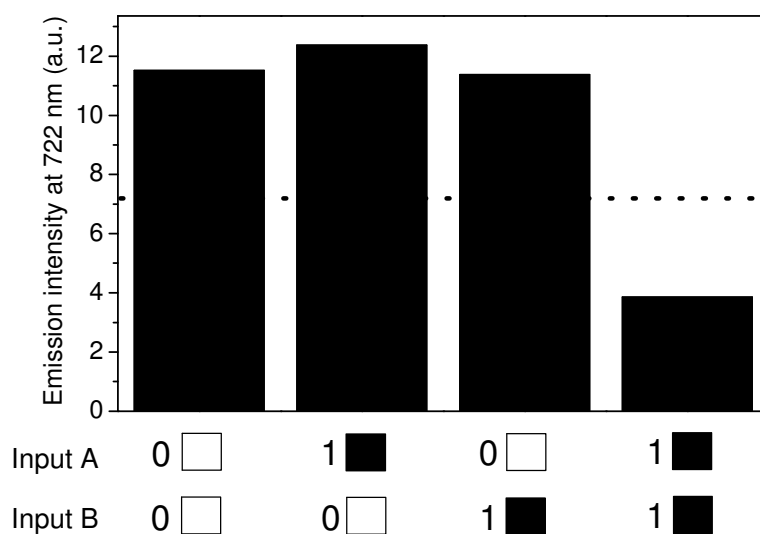
Figure 5. Performance of dyad 1 in the NAND gate mode. The bars show the emission intensity of the porphyrin unit measured at 722 nm after each input combination (see text for details). The sample was excited at 590 nm. The dotted line represents an arbitrarily set threshold level to distinguish output on from output off . Before each input combination, the sample was reset to the initial 1a state.
