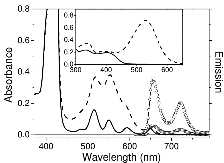
Figure 1. Absorption spectra of solutions dyad 1 in the closed 1a (—) and highly enriched in the open 1b (---) forms. Also shown are the porphyrin emission spectra of these solutions with the dyad in the closed (○-○-○) and highly enriched in the open (□-□-□) forms after excitation at 590 nm. The inset shows the corresponding absorption spectra of the closed 2a (—) and the open 2b (---) forms of the model monomer.
