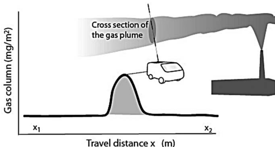
Figure 2. The SOF technique utilizes the absorption of direct solar infrared radiation for retrieval of total columns of various species. The total gas flux emerging from an industrial source is obtained by conducting a downwind transect across its plume and then multiplying the integrated concentration by the plume wind speed.
