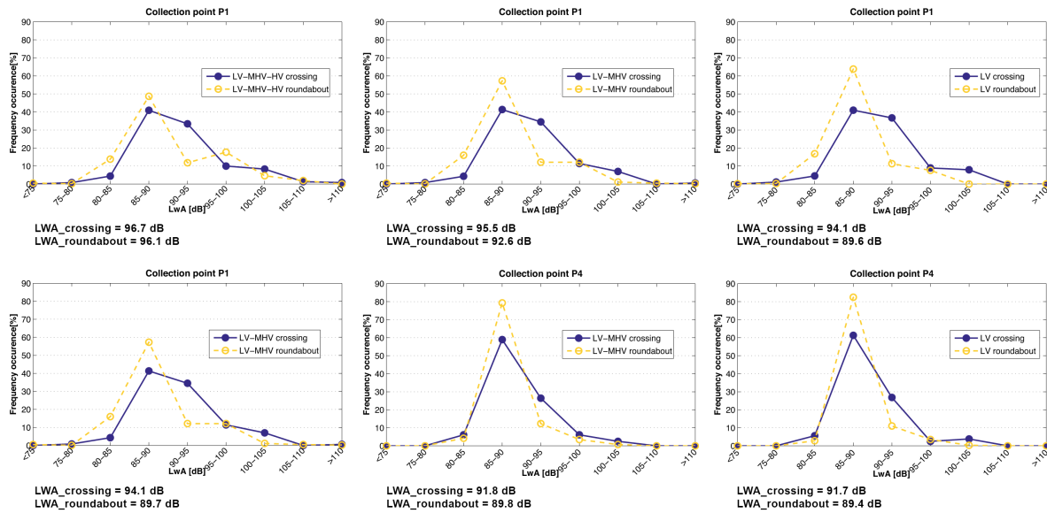
Figure 8 – LWA (dB) at collection points 1 and 4 for the signalized crossing and the roundabout in all cases. Average LWA is displayed in the plot for each case.
