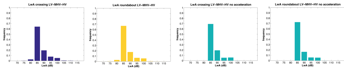
Figure 10 – Sound power level (dBA) at crossing and roundabout network and removing the acceleration effect in both intersections
