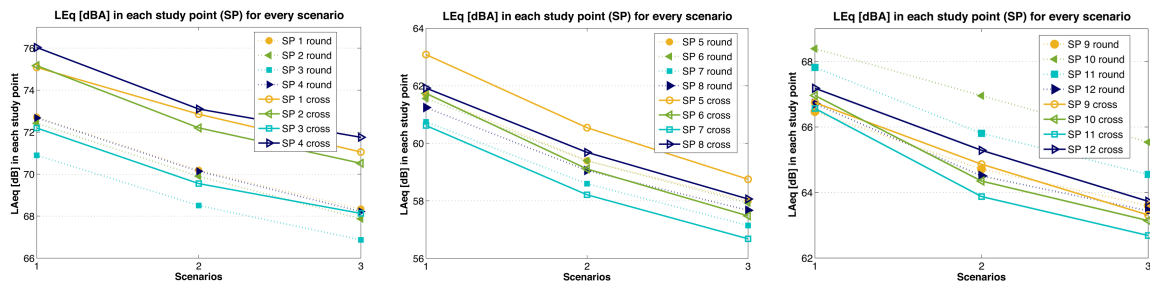
Figure 6 – L_{Aeq} (dB) in each study point for the signalised intersection and the roundabout cases
