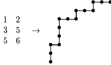
FIGURE 5. An illustration of Theorem 10 for n = 7 .
