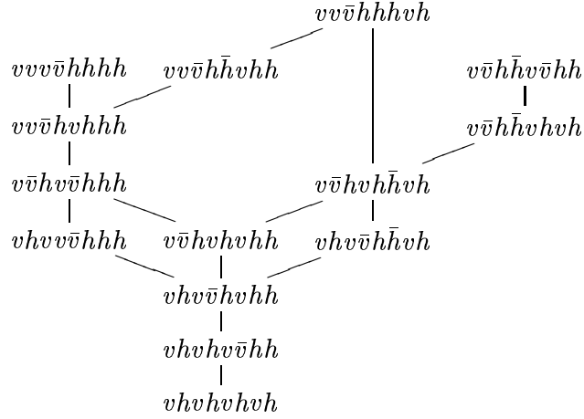
FIGURE 2. The partial order \Omega on \mathcal{D}_4 , with long non-final sequences marked with bars.
