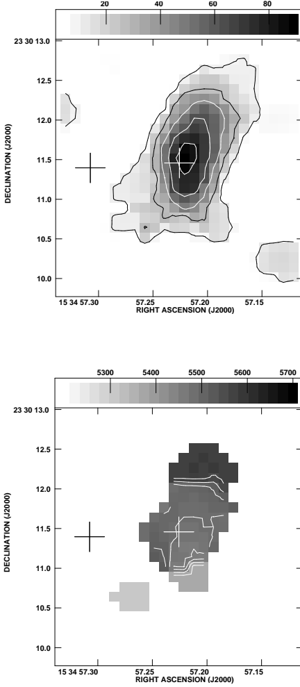
Fig. 4. Top panel: Tapered integrated HNC 3–2 line emission (beam 0.''77 \times 0.''67 with PA=20^\circ ). The grey scale ranges from 5 to 90 \text{Jy beam}^{-1} \text{ km s}^{-1} . Contour levels are 9.0 \text{ Jy beam}^{-1} \text{ km s}^{-1} \times (1, 3, 5, 7, 9) . The rms noise in the map 10 \text{ Jy beam}^{-1} \text{ km s}^{-1} making the first contour 0.9\sigma and the second 2.7\sigma . Crosses mark the position of the 277 GHz continuum peaks. Lower panel: Tapered velocity field. The grey scale ranges from 5200 to 5700 \text{km s}^{-1} and the contours range from 5300 to 5490 \text{km s}^{-1} with steps of 27 \text{ km s}^{-1} .
