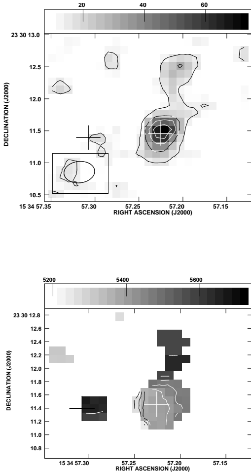
Fig. 1. Top panel: Integrated HNC 3–2 line emission (naturally weighted). The grey scale ranges from 10 to 73 \text{Jy beam}^{-1} \text{km s}^{-1} . Contour levels are 7.3 \text{ Jy beam}^{-1} \text{km s}^{-1} \times (2,4,6,8) . Crosses mark the position of the 277 GHz continuum peaks. The synthesized beam is indicated in the box in the lower left corner. Lower panel: The HNC 3–2 velocity field. The grey scale ranges from 5200 to 5720 \text{km s}^{-1} and the contours range from 5252 to 5616 \text{km s}^{-1} with steps of 52 \text{km s}^{-1} .
