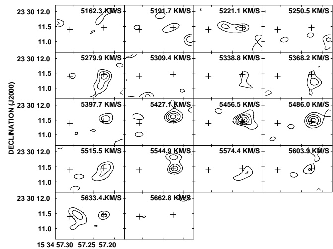
Fig. 3. Naturally weighted channel maps, not smoothed in velocity. Crosses mark the radio continuum positions of the two nuclei. Contour levels are 49 \text{ mJy} \times (2,3,4,5,6) . Peak flux is (330 \pm 50) \text{ mJy/beam} .
