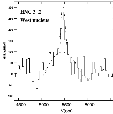
Fig. 2. HNC J=3-2 spectrum of the western nucleus of Arp 220. The spectrum has been Hanning smoothed resulting in a reduced intensity in the narrow component. The spatial resolution is 0.''48 \times 0.''32 . The broad and narrow components are marked with a dashed curve.
