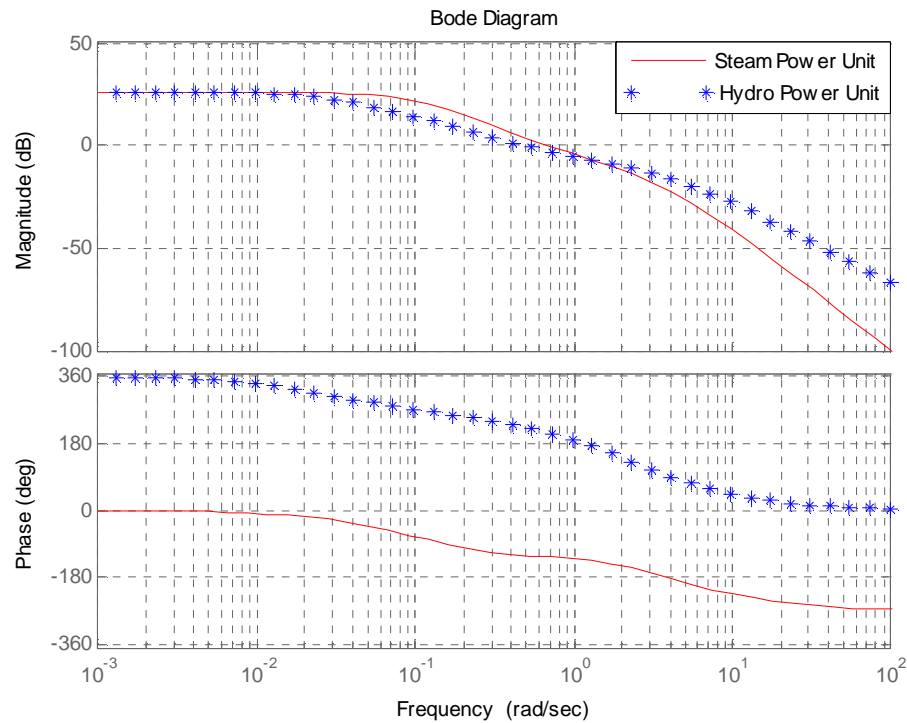
Fig.- 3.29 Gain and phase margins of steam Power Plant and Hydroelectric power plant where no minimum phase shift in magnitude plot.
