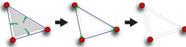
Figure 2 Illustrating the algorithm. Step 1: tension from the membrane is added on to the links, step 2: forces in the links is added to the nodes. Then the nodes have all the information needed to calculate their new positions.
