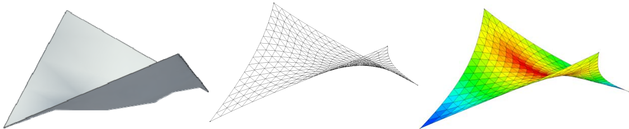
Figure 3. From the left: starting geometry, form found shape, and the structure analysed with 1 kN pressure load applied (the colours are visualizing the warp stress)
