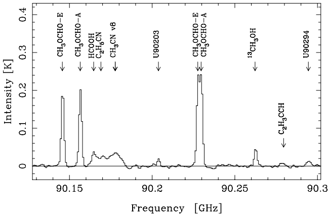
Fig. 1. A part of the observed spectrum towards Orion KL after 31 h of on-source integration. The noise level is \sigma = 2.7 mK. The expected position of one of the vinyl acetylene lines is marked ( C_2H_3CCH ), as well as identifications of other detected lines.
