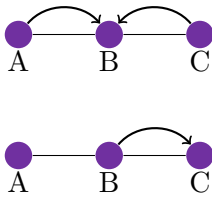
Figure 4.2: The path for information to travel to a second order neighbour via two message passing iterations. For information to get from A to C, it must get to B in an intermediate step. Since the message passing iterations has no concepts of direction, some information will be passed from C to B then back to C. Hypothetically this dilutes the information storage of each node.
