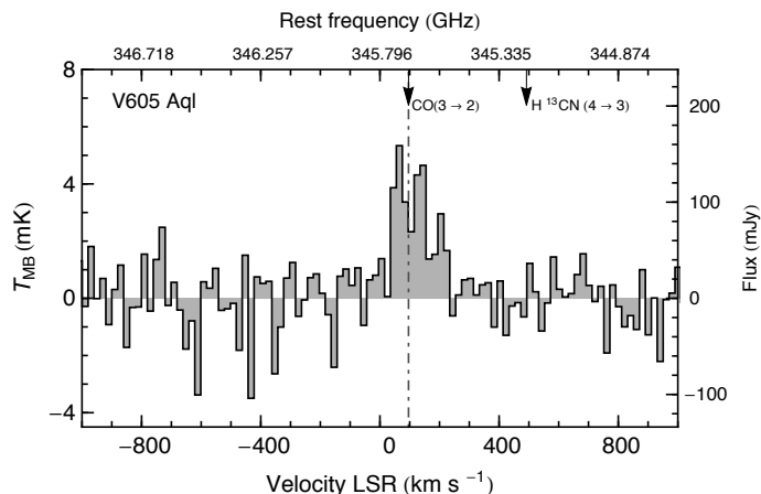
Fig. 3. APEX spectrum of the CO ( J = 3 \rightarrow 2 ) emission in V605 Aql. The width of each channel is 20 \text{ km s}^{-1} . The dotted vertical line corresponds to the systemic velocity relative to the local standard of rest of the PN A58, v_{\text{sys}} = 96 \text{ km s}^{-1} , estimated by Clayton et al. (2013). The arrows indicate the rest frequencies for the CO ( J = 3 \rightarrow 2 ) and \text{H}^{13}\text{CN} ( J = 4 \rightarrow 3 ) lines. The flux density in the right axis was calculated using the corresponding value of \Gamma , shown in Table 1.
