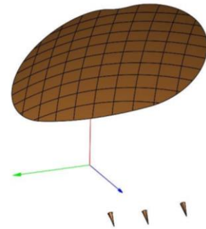
Fig. 4. Torus push-broom antenna with projected aperture D of 5 m, three feeds located at 0 and \pm 20 , f/D=1 , and swath of 600 km.
