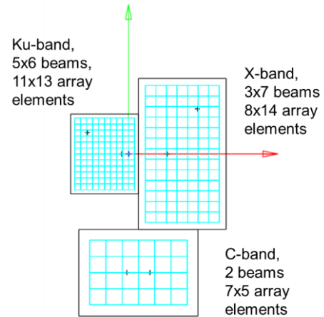
Fig. 5. Feed arrays located in the focal plane.
