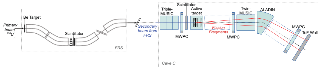
Figure 1. Experimental set-up : production and selection in the FRagment Separator (FRS) of the secondary beam, SOFIA set-up at Cave C.
