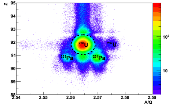
Figure 2. Correlation of the nuclear charge with the ratio of the mass over the charge state for the secondary beam, allowing the identification of the ^{236}\text{U} secondary beam.
