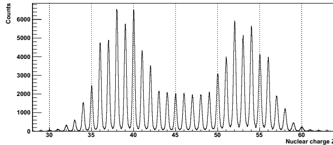
Figure 3. Fission fragments nuclear charge distribution for the electromagnetic-induced fission of ^{236}\text{U} .
