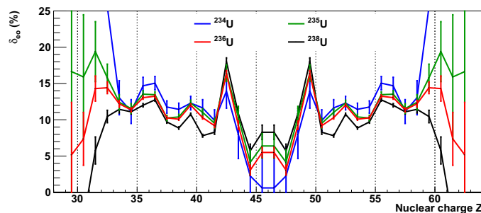
Figure 5. Local even-odd staggering in nuclear-charge yields as a function of the nuclear charge of the fission fragments, for the electromagnetic-induced fission of different U isotopes measured with SOFIA in 2012 for ^{234,235,238}\text{U} and in 2014 for ^{236}\text{U} .
