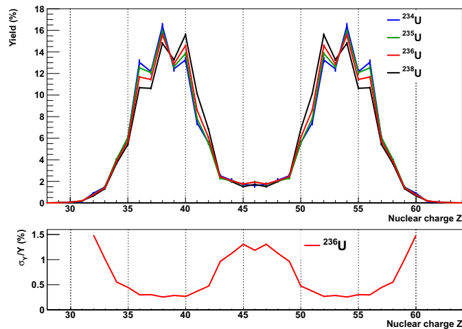
Figure 4. Nuclear charge yields measured with SOFIA for the electromagnetic-induced fission of different Uranium isotopes (top). Relative statistical uncertainty on the elemental yields for the electromagnetic-induced fission of ^{236}\text{U} (bottom).
