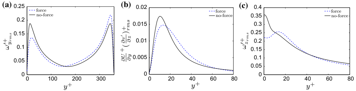
Fig. 20 Wall-normal fluctuation vorticity, \omega'_{y_{rms}} , a \omega'_{y_{rms}} source term, \frac{\partial U}{\partial y} + (\frac{\partial v'}{\partial z})_{rms}^+ , and spanwise fluctuation vorticity, \omega'_{z_{rms}} . Re_\tau = 400 , St = 80\pi . a Wall-normal fluctuation vorticity, \omega'_{y_{rms}} , b a streamwise vorticity source term, \frac{\partial U}{\partial y} + (\frac{\partial v'}{\partial z})_{rms}^+ , c Spanwise fluctuation vorticity, \omega'_{z_{rms}}
