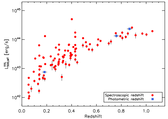
Fig. 5. Distribution of the bright XXL cluster sample in the (z, L_X) plane. The luminosity is measured in the [0.5-2] keV band and integrated to r_{500, \text{MT}} . The data show a clear Malmquist bias due to the flux selection combined with volume effects that prevent us from detecting massive (and thus luminous) clusters at low redshift.
