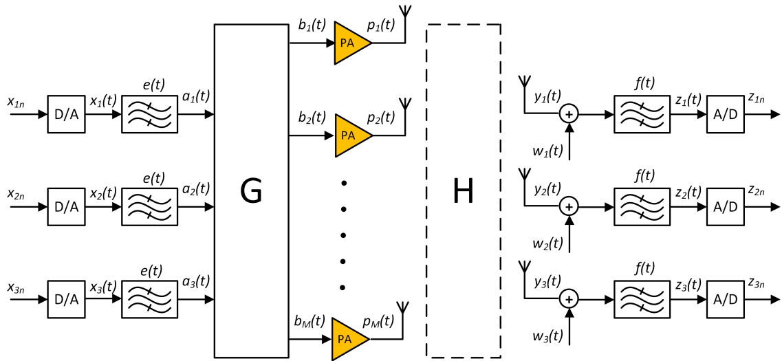
Figure 4.4: Block diagram of the system consisting of M antennas and 3 users.
