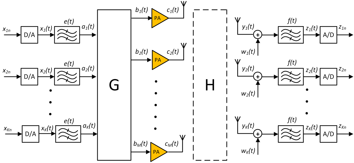
Figure F.1: Block diagram of the system consisting of M antennas and K users.
