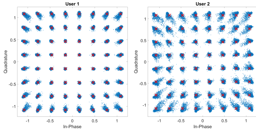
Figure 5.1: Received constellations at each user in a 2x2 scenario. A greater degree of non-linear distortion can be observed for User 2 due to channel conditions.
