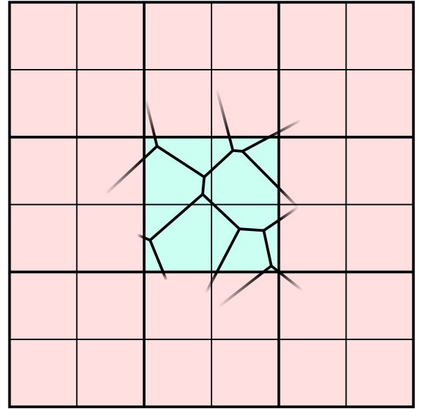
(b) The connectEdges stage is responsible for selecting and storing only the edges that are used by the Voronoi diagram in the green grid cell.
