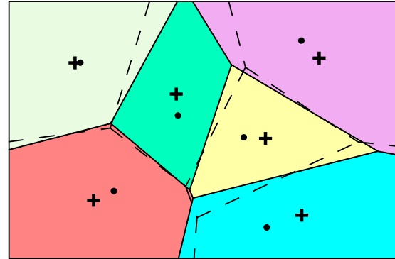
(b) The same diagram with the sites of first iteration of Lloyd's algorithm marked as crosses. The dashed polygons indicate the Voronoi diagram of the new relaxed sites.
