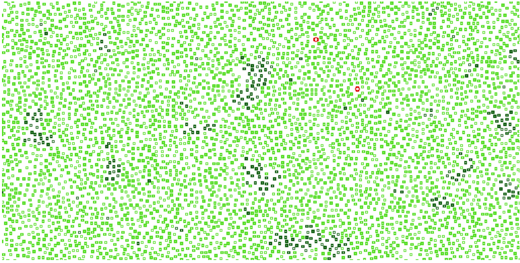
Figure 3.14: Entities distributed using Poisson disc distribution. Light green entities have self spawn chance P_s = 0 chance and population value N = 500 , dark green entities have P_s = 85\% leading to clusters. Red entities have P_s = 0 and N = 1 which can be seen in their low numbers in the figure. Light green entities have the highest population value and subsequently dominate in numbers.
