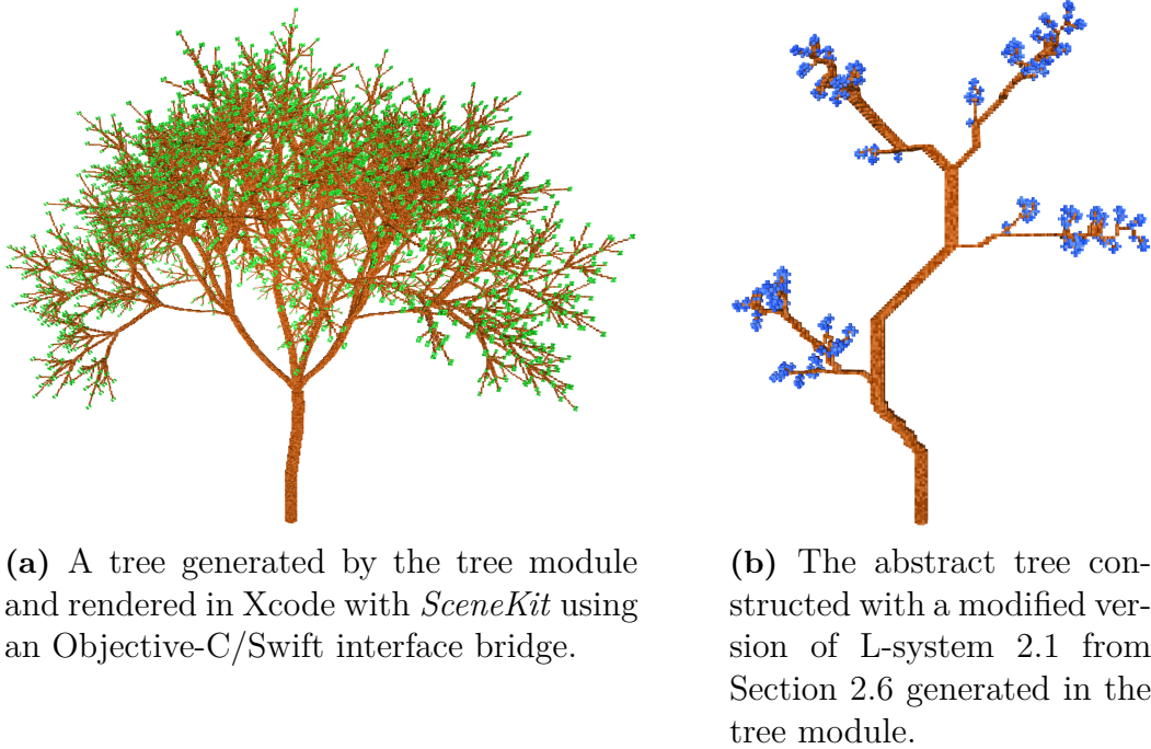
Figure 4.3: The results of the tree module, using L-systems to construct trees.
